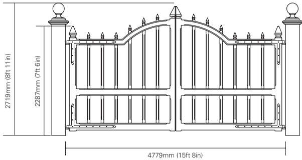
Fig.A entrance gates
