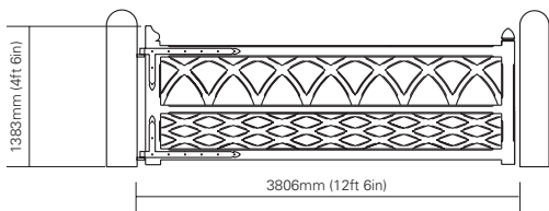
Fig.E victorian lodge gate
