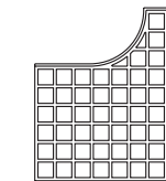
4RB/L drop curve panel 1245 x 1420mm (4ft 1in x 4ft 8in)
