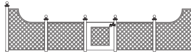
hampton court gate screen 6.5m length 100mm (4in) centres diamond with gate 24 x 11mm batten overlap
