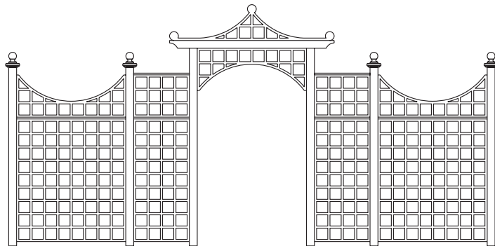
chinese arch screen 5.5m length 152mm (6in) centres square jointed 24 x 22mm batten half-lap jointed
