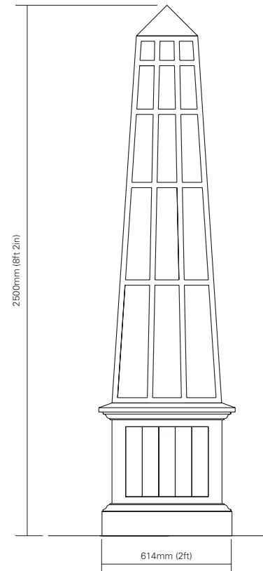
OC/OB/PL obelisk on a planter
