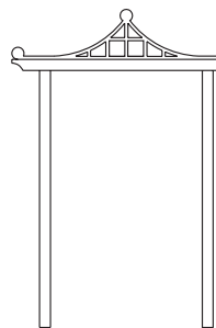
4CHP complete chinese arch opening width 1245mm (4ft 1in) overall height 2600mm (8ft 6in)
