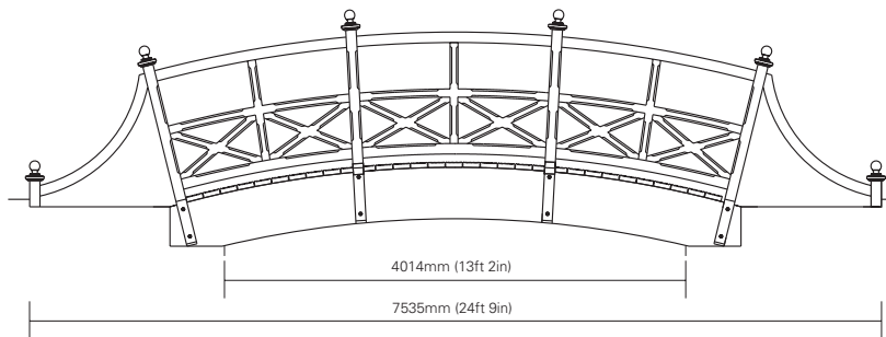
regency style bridge (curved)
