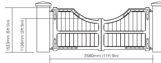
Fig.F close boarded gates
