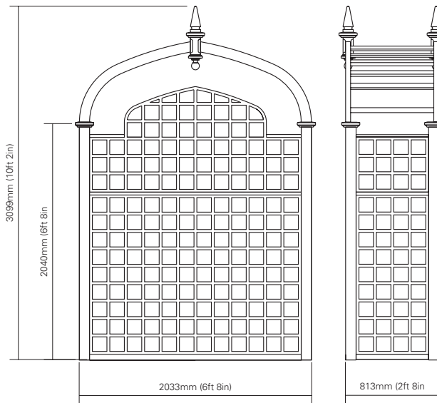
SA/TUD/GOTH 6ft tudor gothic seat arbour
