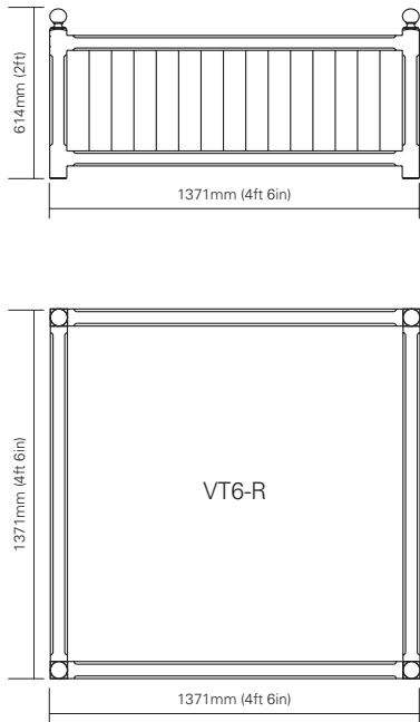
VT6-R extra large shallow planter
