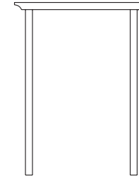
4PLA post and lintel arch opening width 1245mm (4ft 1in) overall height 2340mm (7ft 8in)
