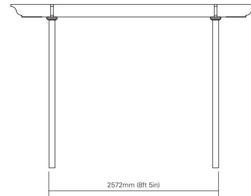
pergola with solid posts
