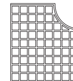
4DB/R drop curve panel 1245 x 1420mm (4ft 1in x 4ft 8in)
