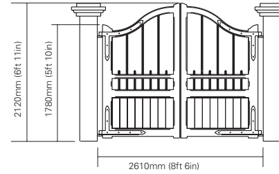
Fig.B serpentine gates with steel bars
