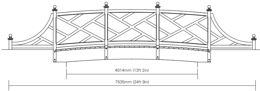
chinese chippendale bridge
