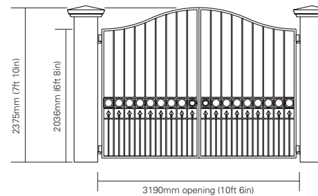
Fig.H steel serpentine entrance gates
