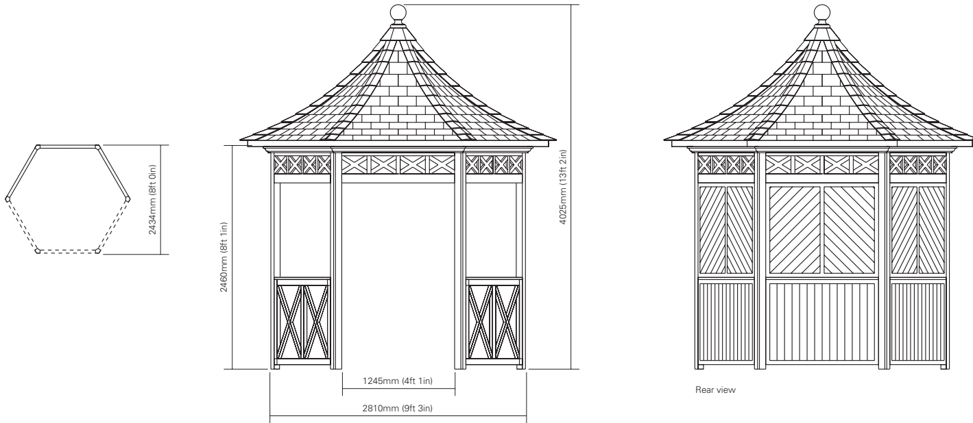
Fig.E hexagonal regency style shingle roof gazebo with boarded sides and back, front open with cross-braced dado panels
