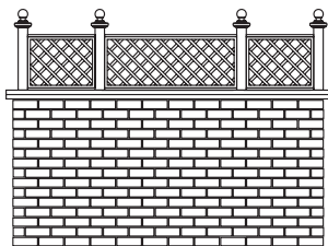
diamond trelliswork on a wall 2.9m length (optional post shoes NOT included) 100mm (4in) centres diamond 24 x 11mm batten overlap
