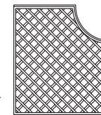
D-4DB/R diamond drop curve panel 1245 x 1420mm (4ft 1in x 4ft 8in)
