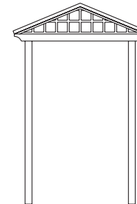
4CPA complete classical arch opening width 1245mm (4ft 1in) overall height 2600mm (8ft 6in)
