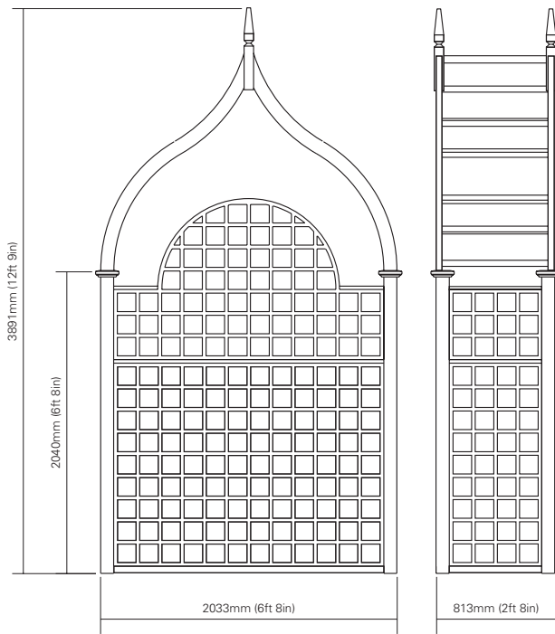
SA-GOTH 6ft gothic seat arbour
