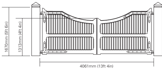
Fig.C entrance gates with steel bars
