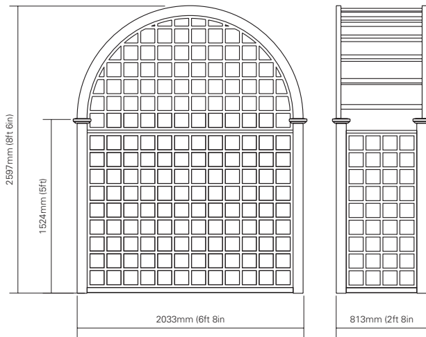
SA-SERP 6ft serpentine seat arbour with square trellis panels (shown)
