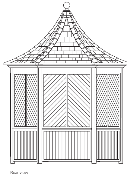
Fig.C hexagonal shingle roof gazebo with three faces boarded, front open with trellis arches and boarded dado panels
