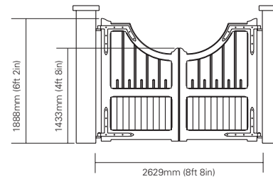
Fig.D lodge gates
