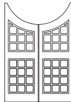
4MG (pair) 4ft moon gates (including standard hardware) 1240 x 1800 x 44mm (4ft 1in x 5ft 10in x 1 3/4in)
