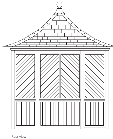
Fig.D square shingle roof gazebo with boarded sides and back, front open with boarded dado panels
