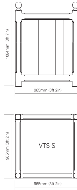
VTS-S extra heavy tree planter
