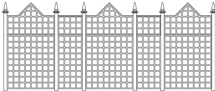
elizabethan screen 5.5m length 152mm (6in) centres square jointed 24 x 22mm batten half-lap jointed
