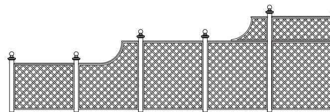
diamond panels showing height increase 6.8m length 100mm (4in) centres diamond 24 x 11mm batten overlap
