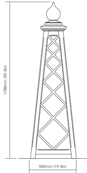
OC/OB/GF obelisk with gothic finial
