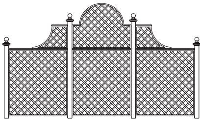
diamond drop curve screen 4m length 100mm (4in) centres diamond 24 x 11mm batten overlap
