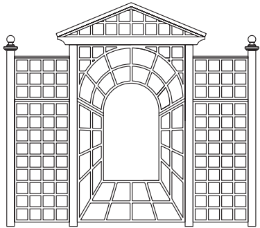
perspective illusion screen 2.9m length 152mm (6in) centres square jointed 24 x 22mm batten half-lap jointed
