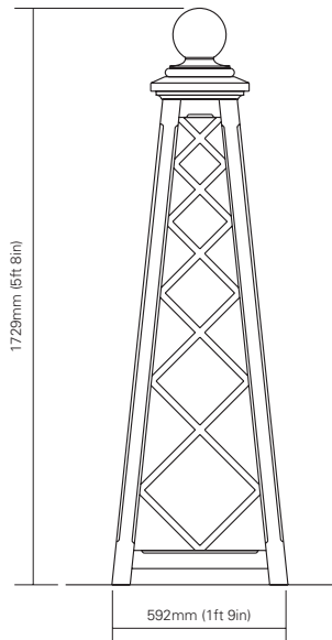
OC/OB/BF obelisk with ball finial
