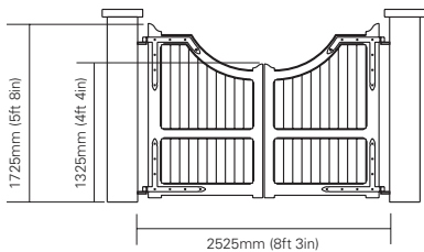
Fig.G close boarded gates
