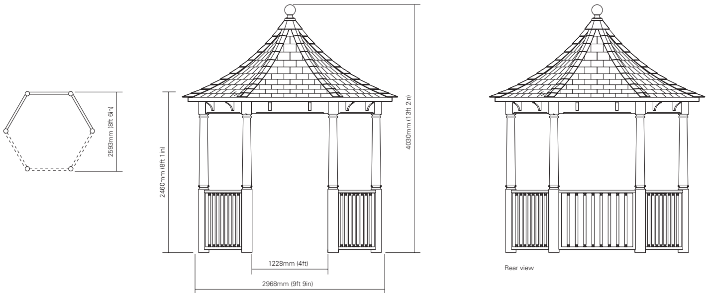
Fig.F hexagonal shingle roof gazebo with tapered columns and dado railing panels
